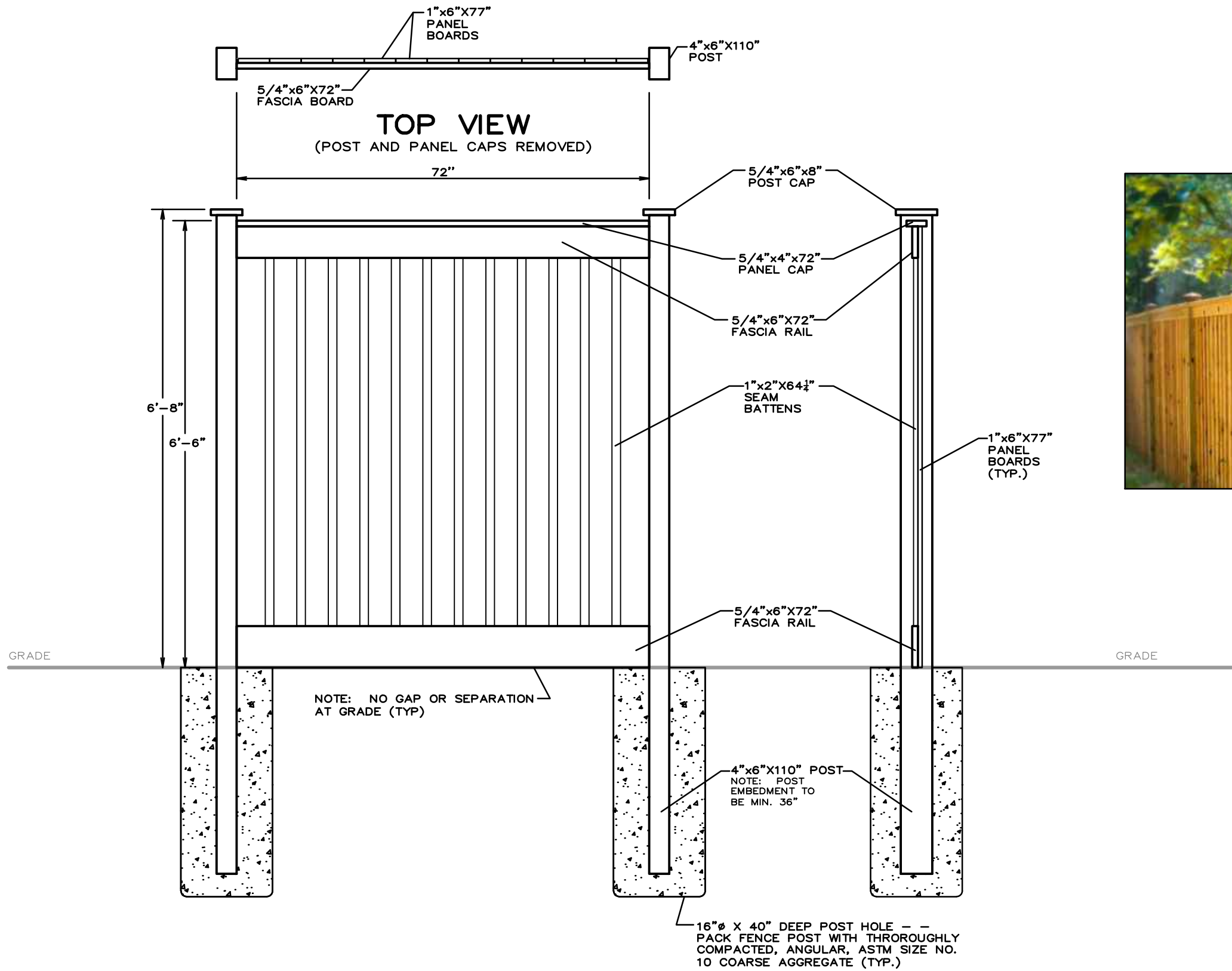
ELEVATION VIEW
